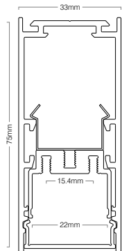
Profile Dimensions
